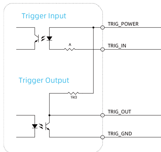
Figure 4 Trigger circuit schematic diagram (falling-edge)
